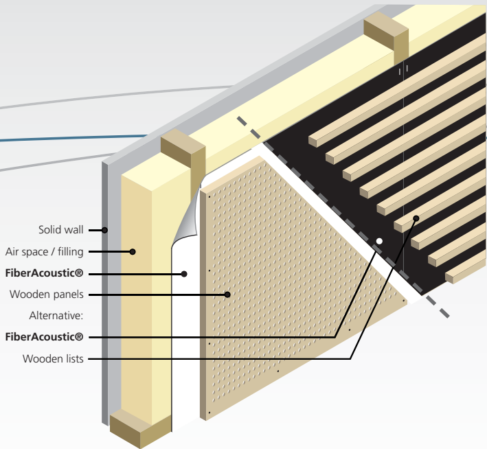
Built up of wooden or steel structure.
