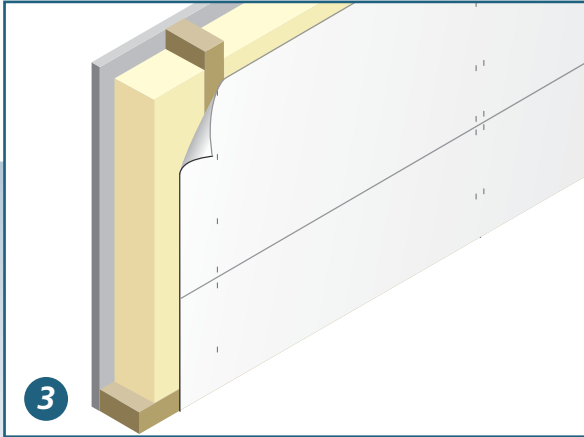
FiberAcoustic® is fastened by clamps, nails, screws or glue.
