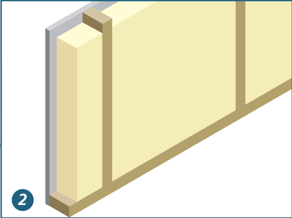
Mineral wool to be installed. It is important that the mineral wool is minimum as thick as the wood/steel laths.
