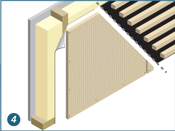
Panels or lists are installed.
